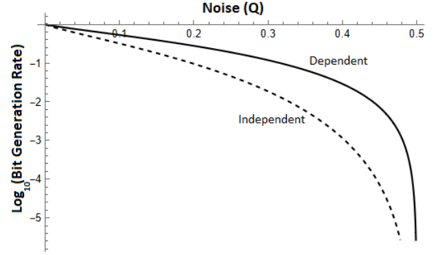
Fig. 2. Showing the bit-generation rate of our SQRNG protocol under depolarization noise. Both the dependent and independent channel cases are plotted.
